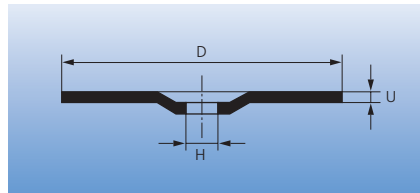
Depressed centre type
